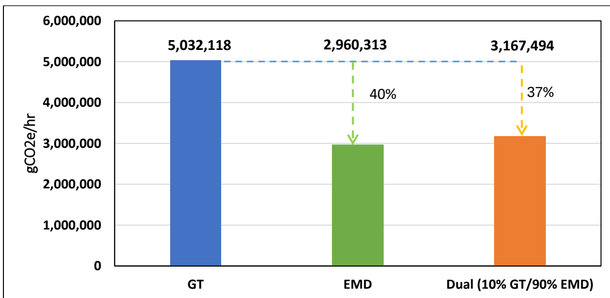
Figure 21 - Comparison of Green House Gas Emissions from One Compressor by Fuel Type
